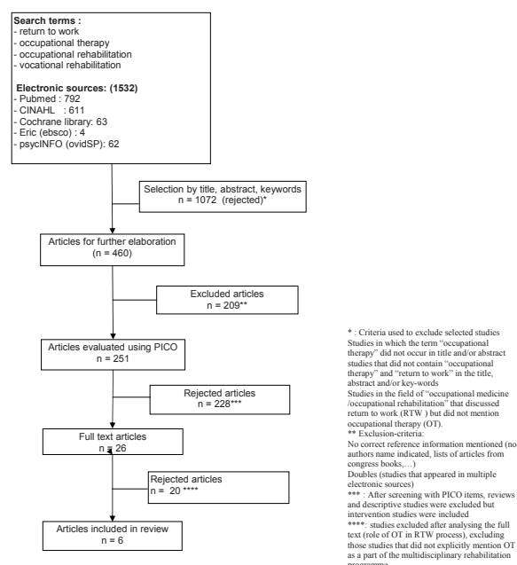
Figure 1: Search strategy .
